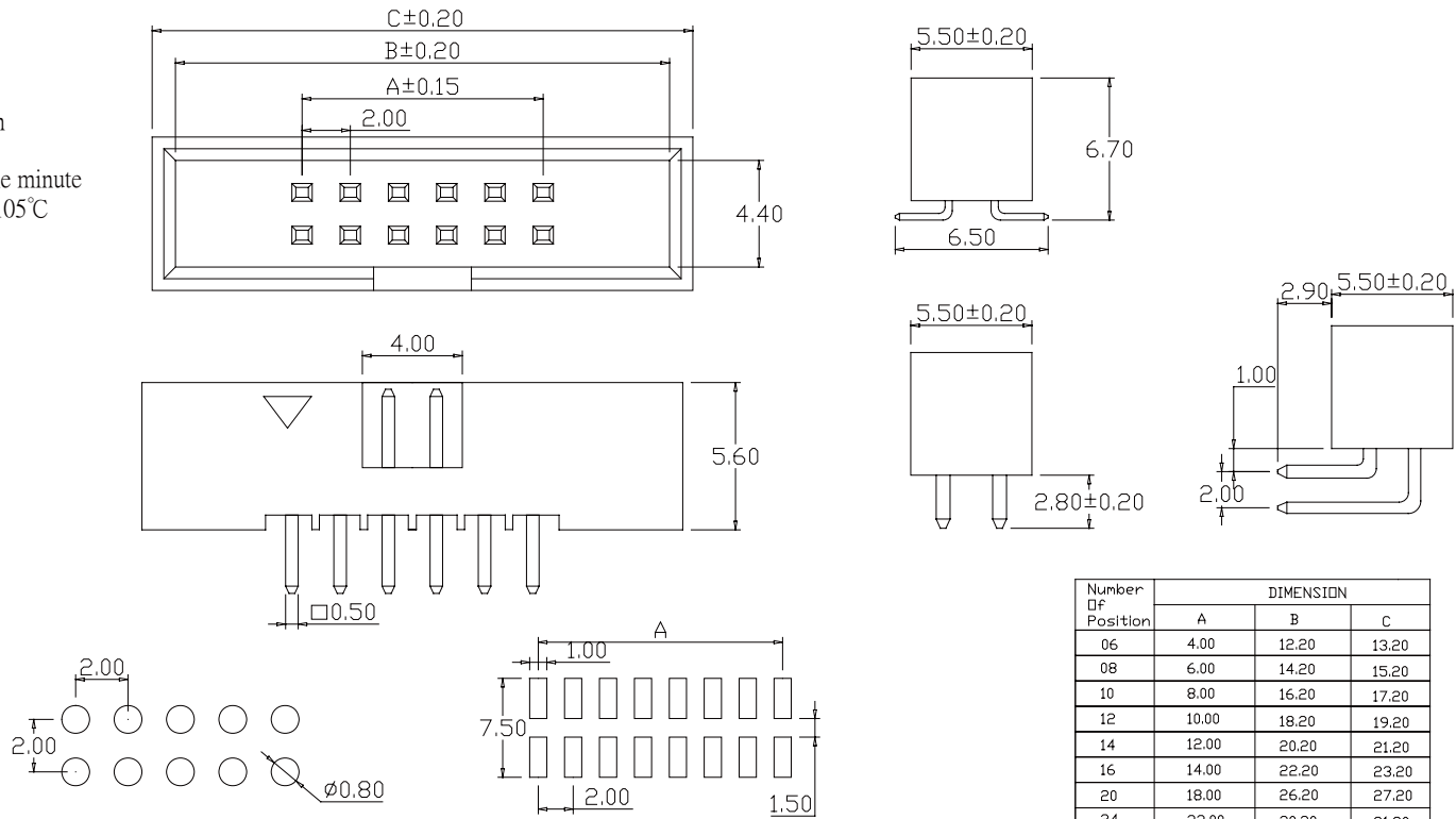
Recommended PCB Layout (PCB TOLERANCE±0.05)
